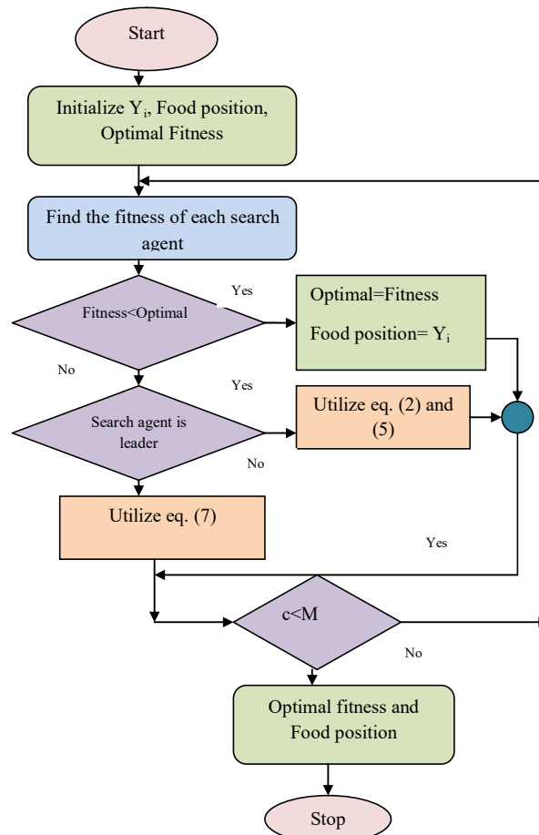
Fig. 3. Flow chart of the proposed ISSA algorithm
