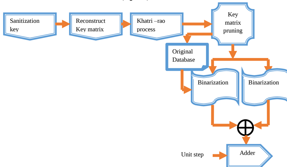
Fig. 2. Diagrammatic representation of the sanitization process
