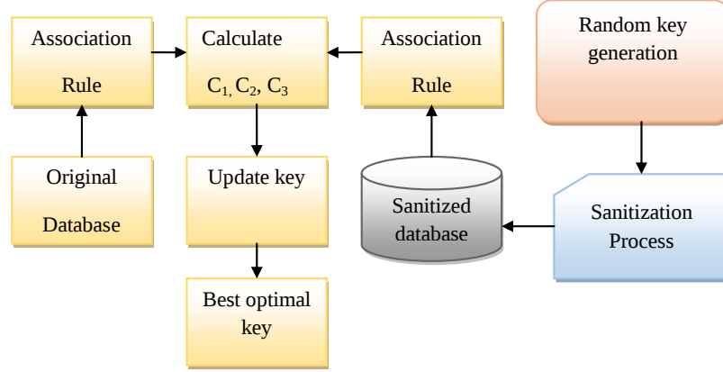
Fig. 3. Architecture diagram of the key generation process
