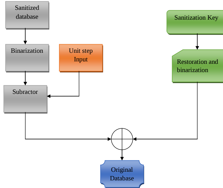
Fig. 4. Schematic diagram of the decoding process
