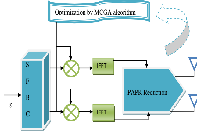
Fig. 1. Block diagram of proposed MCGA base-scrambling approach.
