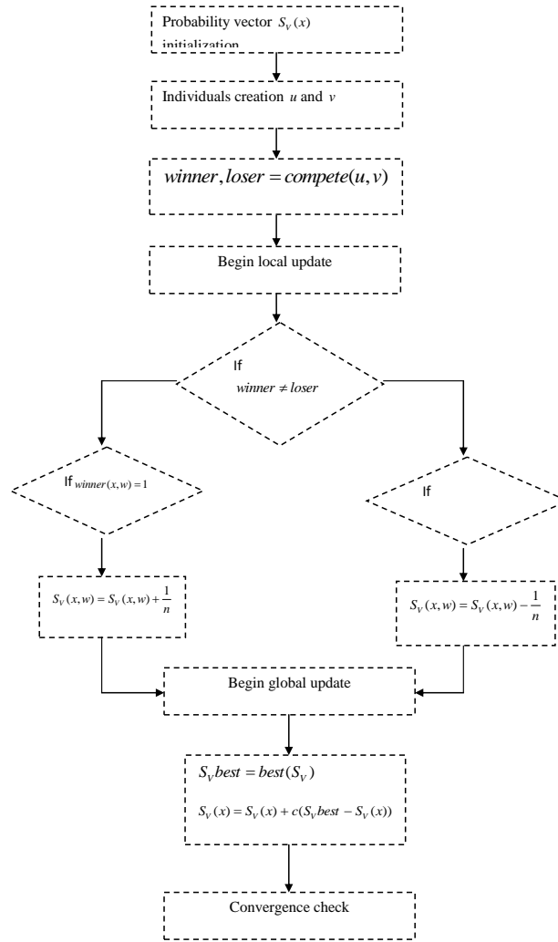
Fig. 2. Flowchart of MCGA algorithm
