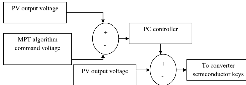
Fig. 1. Control model of PV array
